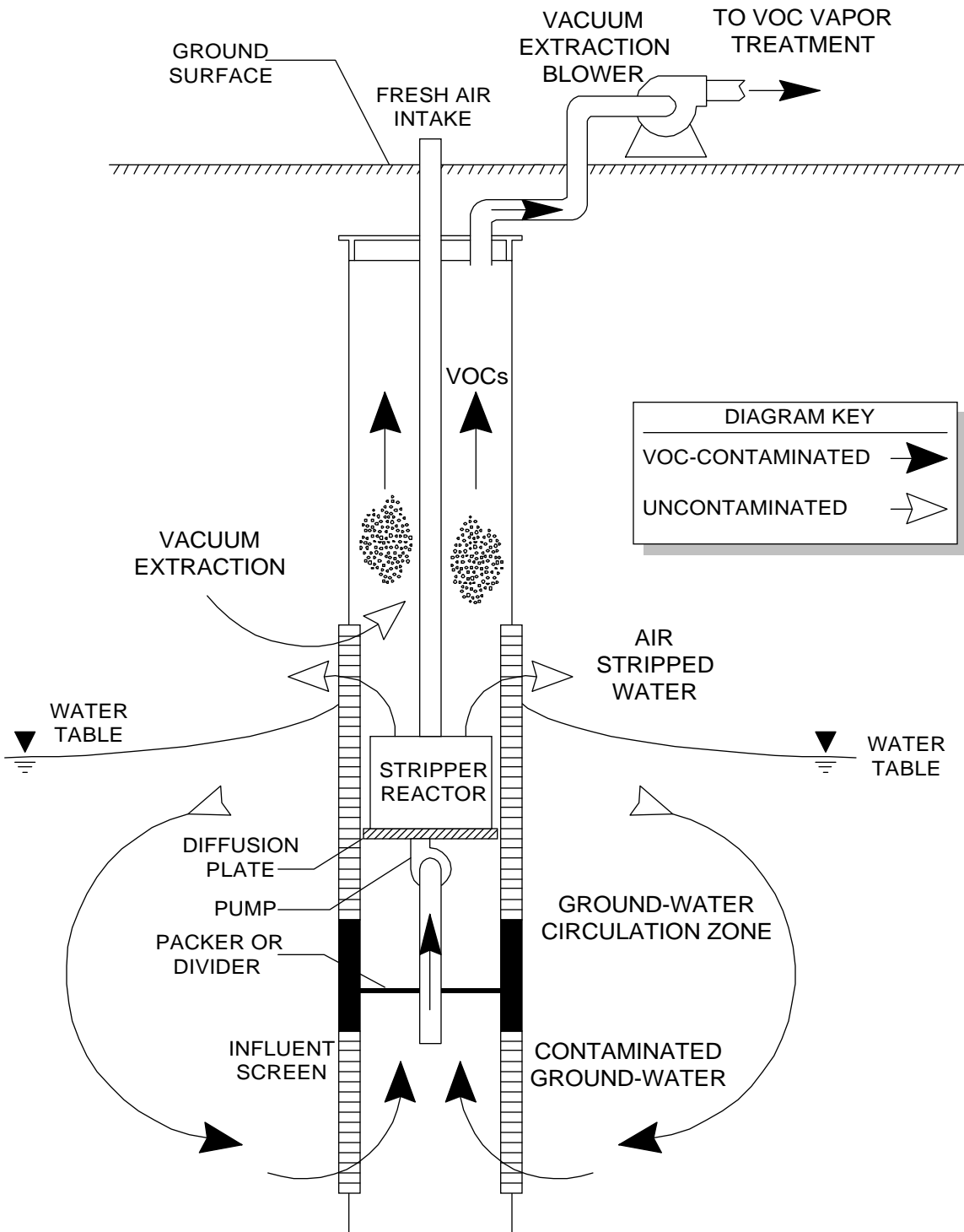
FIGURE 3. UVB IN-WELL VAPOR STRIPPING PROCESS
